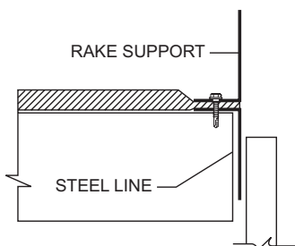
PREPARING PANEL FOR SEAMER WITH HAND TOOL
