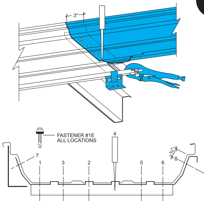
FASTENER SEQUENCE FIRST RUN - ENDLAP
