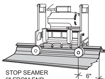
FLATTENING MALE LEG BEFORE PANEL INSTALLATION
