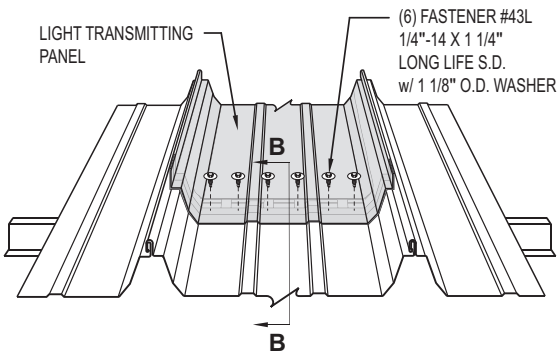
DOWN SLOPE END OF LTP PANEL
